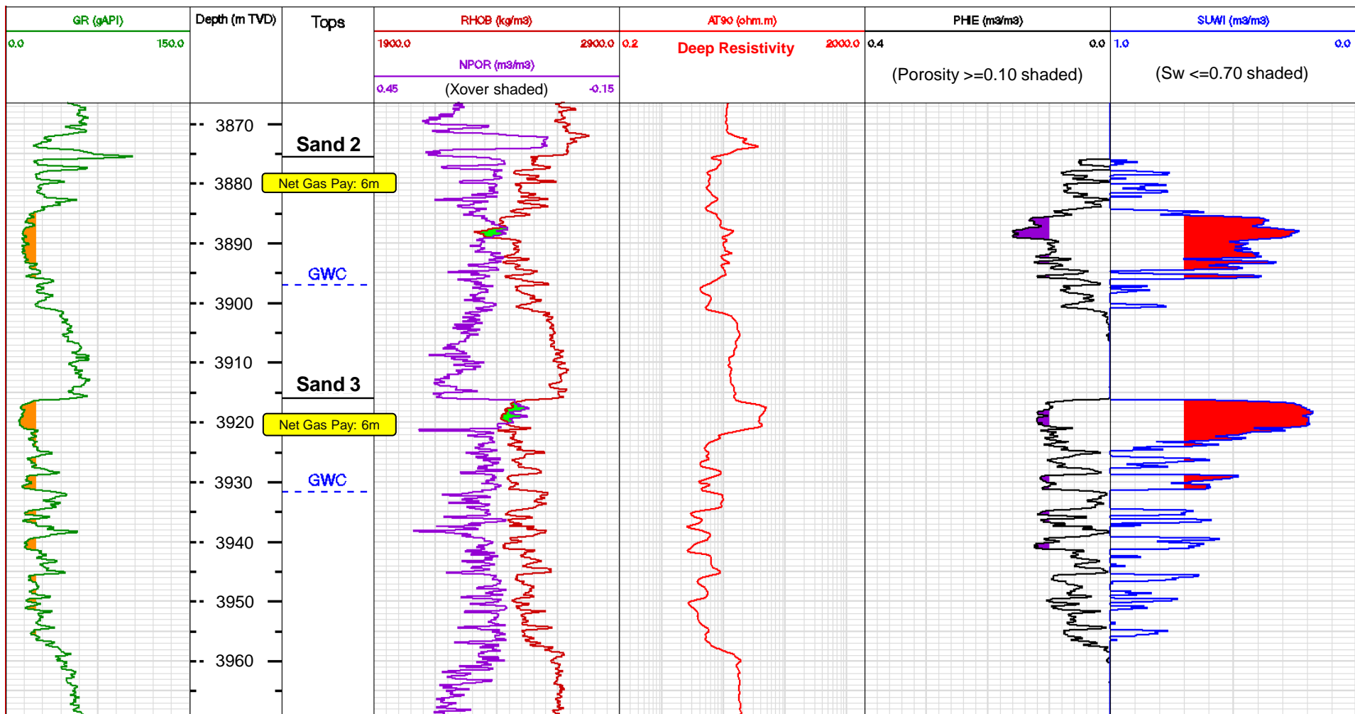
Adamant N-97 – Sands 2 & 3 (Lower Missisauga) Petrophysical Results Plot. Note each sand has six metres of net gas pay over water.
